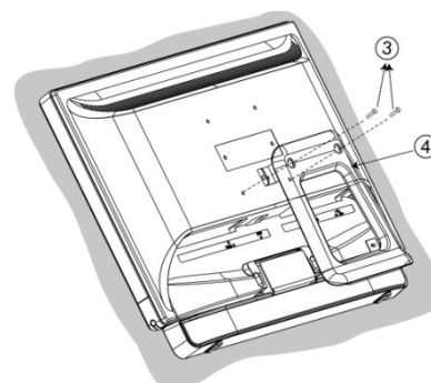
100mm x 100mm Screw Mounting Options
