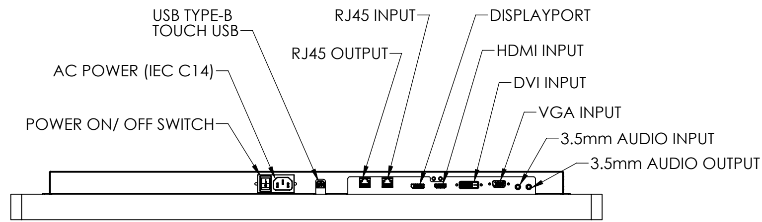
BOTTOM VIEW
