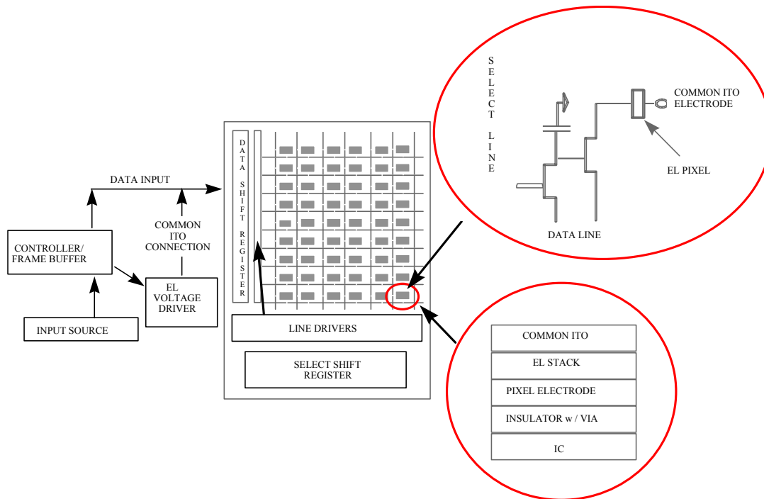
Figure 9: Diagram of AMEL Display Organization
