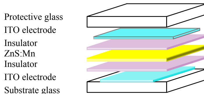
Figure 12: Schematic Diagram of Transparent TFEL Structure
