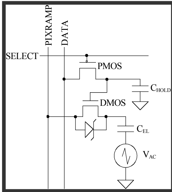
Figure 11: Analog AMEL Pixel Design
