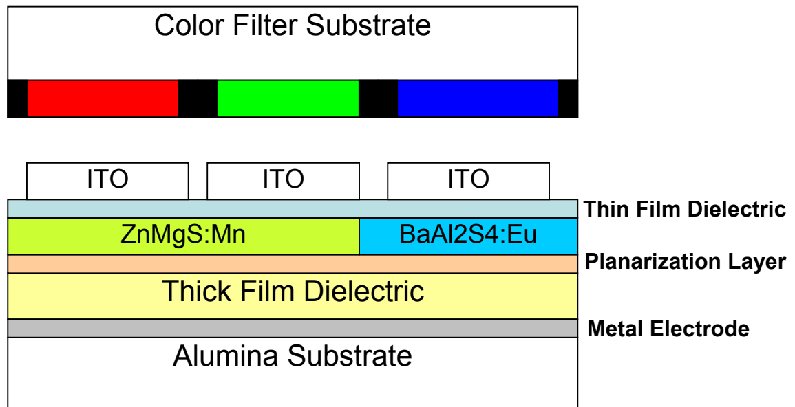
Figure 8: Diagram of 2-Phosphor Color TDEL Structure
