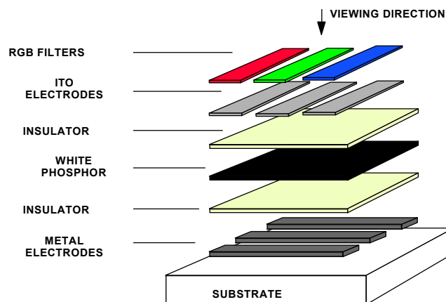
Figure 7: Diagram of Color by White Structure
