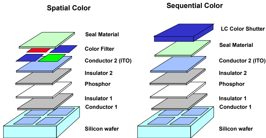
Figure 10: Color AMEL Display Structures
