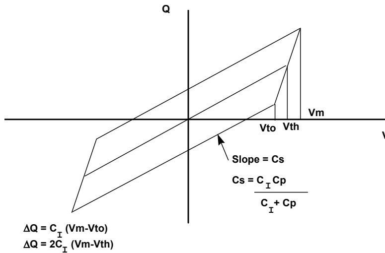
Figure 4: Q-V Characteristic of an EL Device
