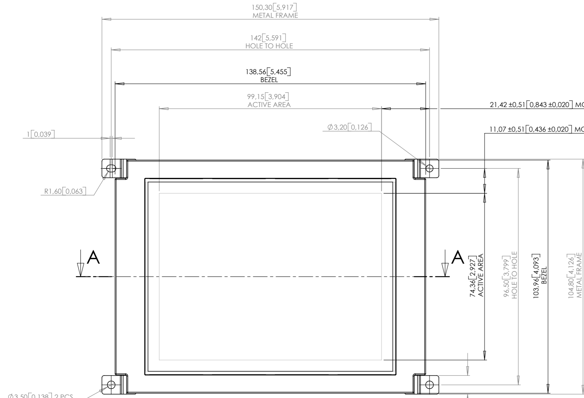
FRONT VIEW
